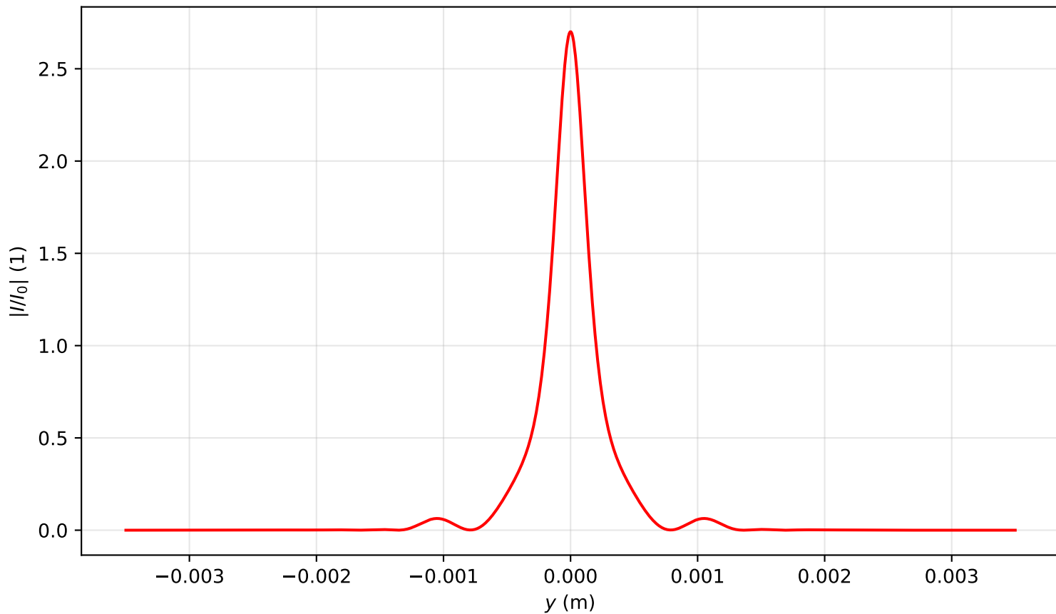
Intensity profile I(x = 0, y, z = 1.672)/I_0 , P_{in}=2.5P_{cr} , artificial time
